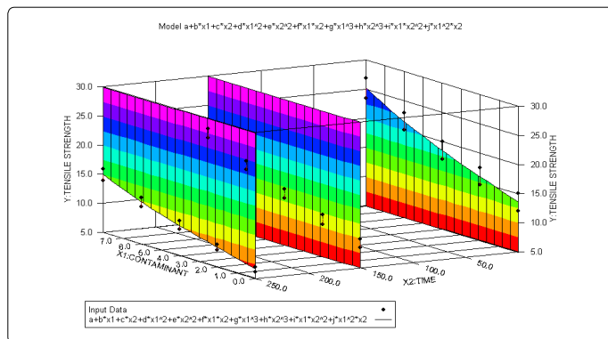
Figure 4. Indicate a theoretical model data for RLDPE of both Iraqui and Foreign waste
