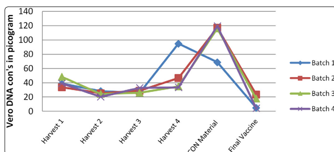
Figure 3b. Residual vero cellular DNA in different stages of purification estimated by real time PCR.
