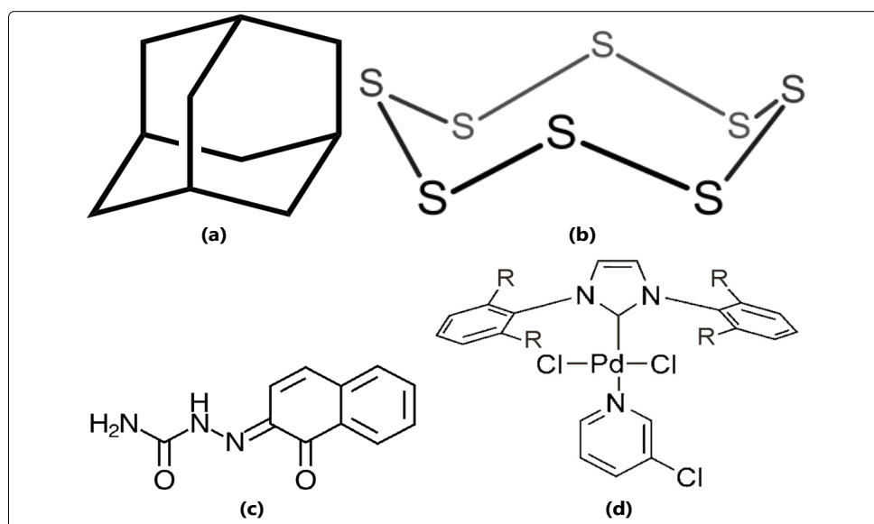
Figure 1. Molecular structure of (a) Adamantane, (b) Irene, (c) Naftazone and (d) PEPPSI Nano molecules.
