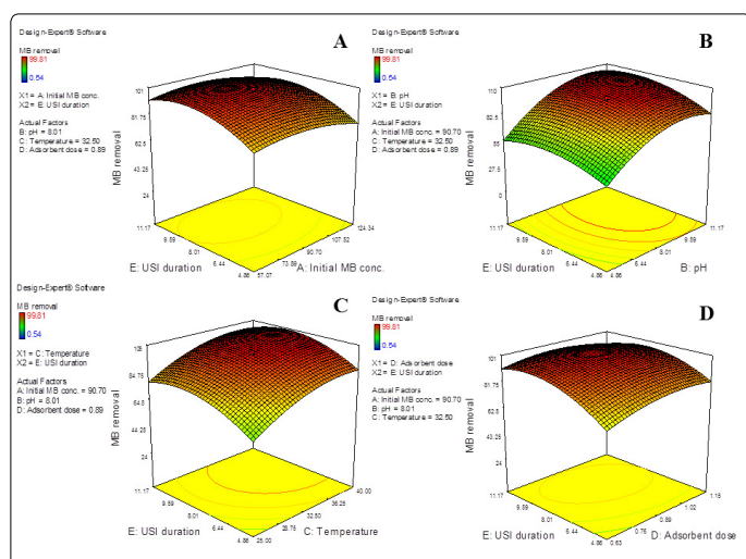
Figure 3. 3D plots obtained from RSM (CCD) analysis showing effect of independent variables with respect to duration of ultrasonic irradiation (USI) on MB adsorption using GO- ZnO NP composite. Figures A–D represent interactions of duration of USI with varying initial MB concentration, solution pH, ambient temperature and adsorption dosage respectively on the process of adsorption reported in this study.
