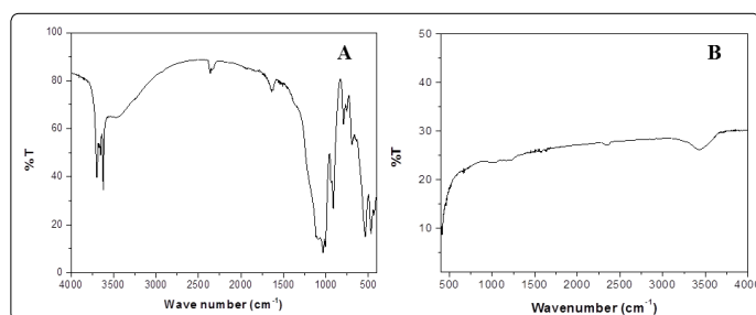
Figure 5. FTIR spectrum of GO- ZnO NP composite before (spectrum A) and after (spectrum B) adsorption.
