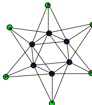
Figure 6. Isomeric skeletal structure of \text{Ir}_{12}(\text{CO})_{24}^{2-} .
