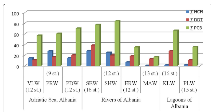
Figure 1. Total of HCHs, DDTs and PCB markers in water samples ecosystems
