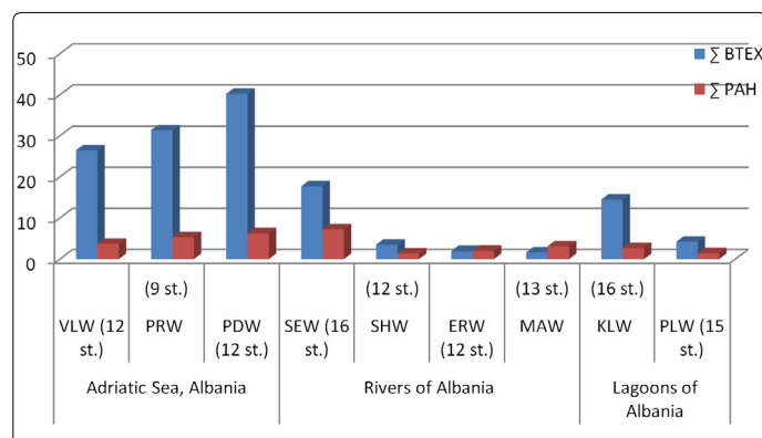
Figure 2. Total of PAHs and BTEX in water samples ecosystems
