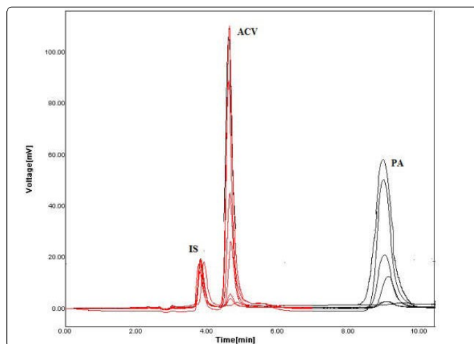
Fig. 6. Overlaid chromatograms illustrating the calibration curves of ACV and PA binary mixtures spiked in rabbit plasma in concentration ranges of 0.5-30 µg/ml of each drug in the presence of 2µg/ml of IS
